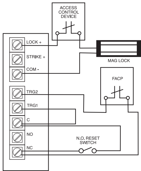
Fig. 5 - Latching fire alarm tie-in with manual reset:
