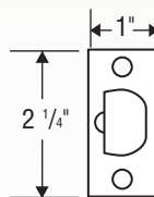
Dead Latch
