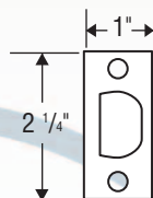
Spring Latch
