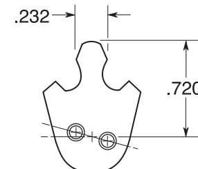
C161 (when ordered with cylinder, step E, page 2) 1E - C161 (for cam only)
