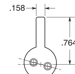
C210 (when ordered with cylinder, step E, page 2) 1E - C210 (for cam only)
